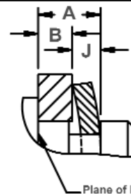
Outer Groove Wall Location A max=B min + J max A min=B max + J min
